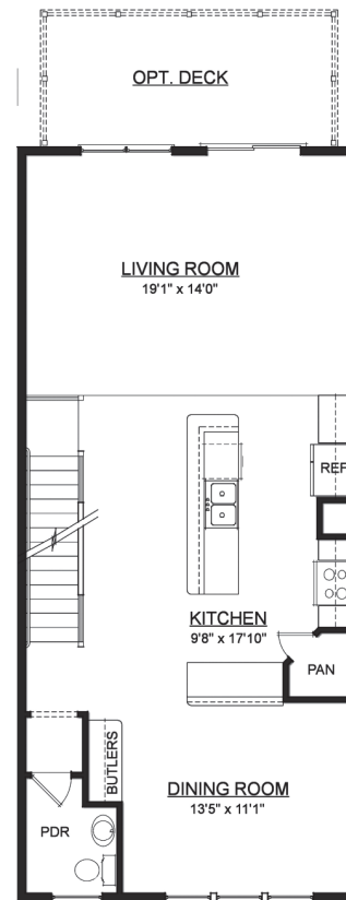
2 ND FLOOR PLAN AT UPPER LEVEL MASTER
